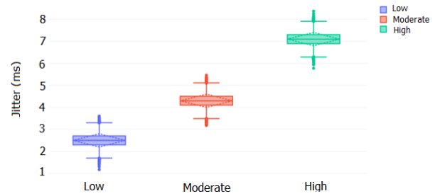
Fig. 3. Jitter distribution in Wi-Fi 7 by density.
