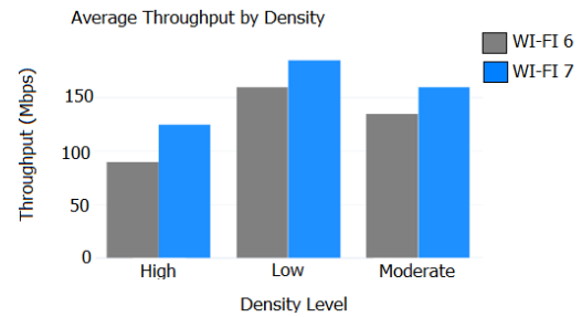
Fig. 1. Throughput comparison of Wi-Fi 6 vs. Wi-Fi 7 across density levels.
