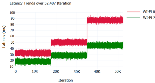
Fig. 2. Average latency for Wi-Fi 6 and Wi-Fi 7 under varying density.
