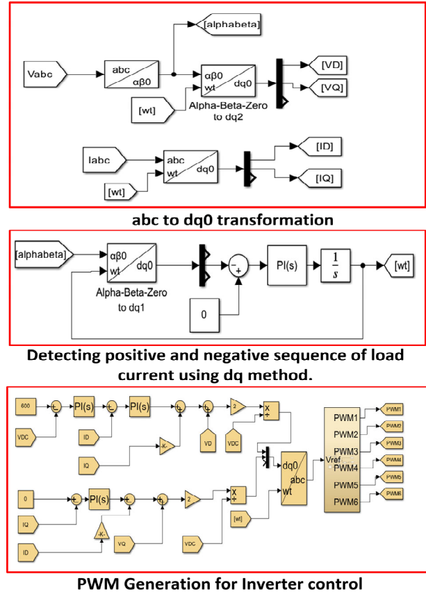
Fig. 9. Simulink design of dq controller for the three phase inverter.
