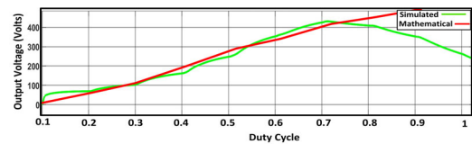
Fig. 5. Comparison of output voltage variation with varying duty cycle of the CCBC with simulated and mathematical analysis.
