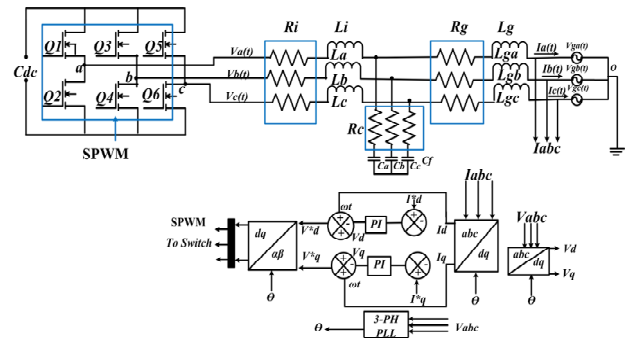
Fig. 8. Three phase full bridge inverter circuit diagram presenting the LCL filter and dq control scheme.
