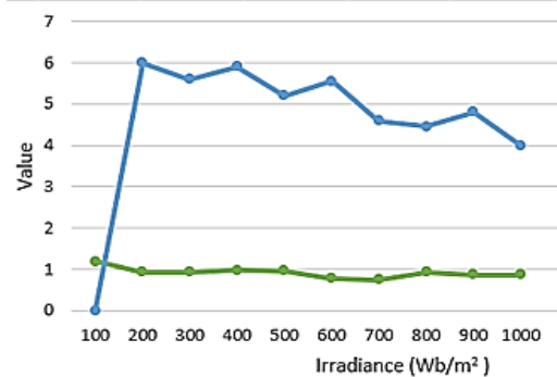
Fig. 16. Input ripple current and output ripple voltage w.r.t variable irradiance.
