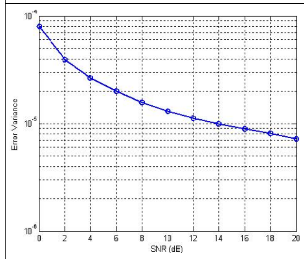
Figure 2: Error Variance of Frequency Offset Estimation Performance in AWGN Channel with QPSK
