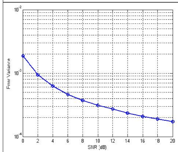
Figure 3: Error Variance of Frequency Offset Estimation Performance in AWGN Channel with 16-QAM
