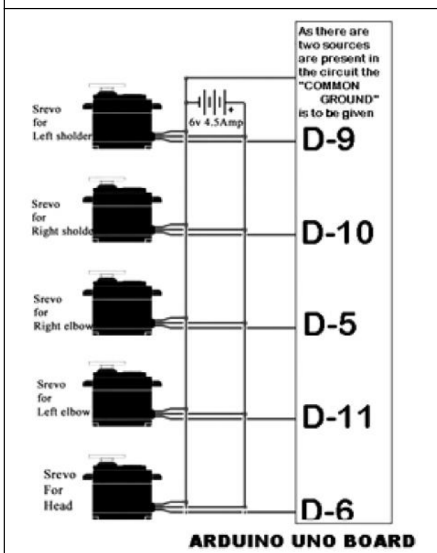
Figure 8: Pin Connections from Arduino to Servos
