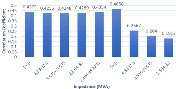
Fig. 3. Correlation coefficient during 5 MVA impedance switching in grid-connected mode.
