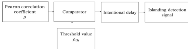
Fig. 2. Block diagram of islanding detection principle.
