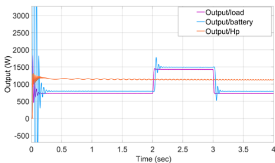
Fig. 9. Output simulation for load, battery, and hydropower.
