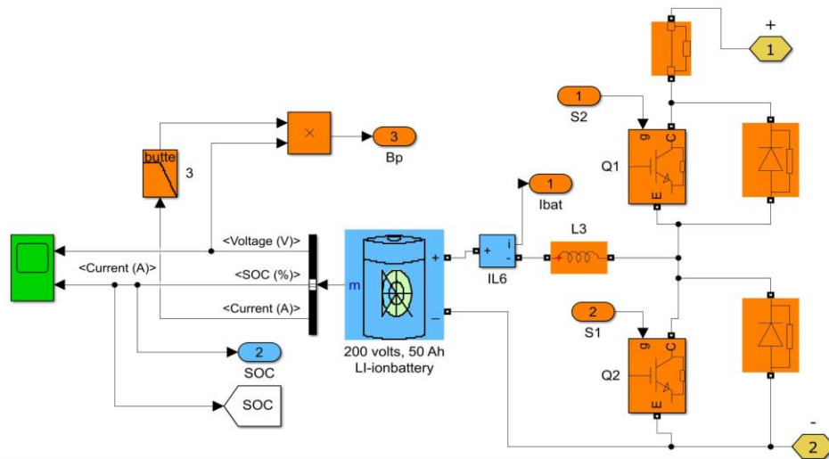
Fig. 4. BESS system with 200V, 50Ah Li-ion battery.
