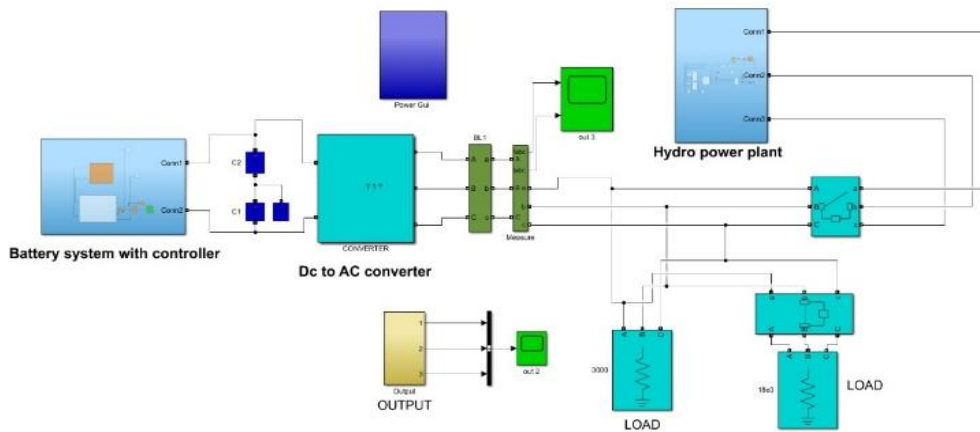
Fig. 3. DC to AC converter in MATLAB Simulink.
