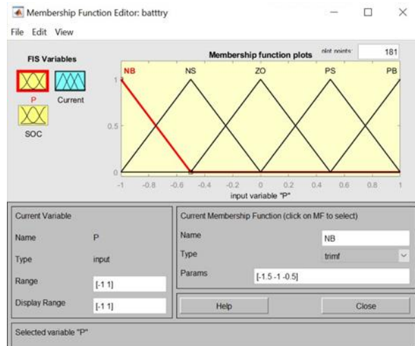
Fig. 6. Membership function for battery controller.
