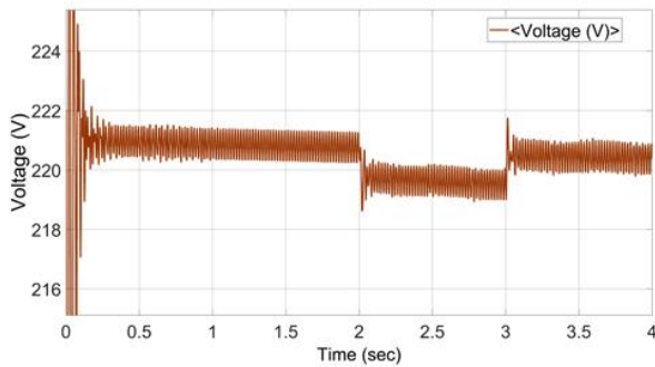
Fig. 7. Simulation analysis for battery voltage.
