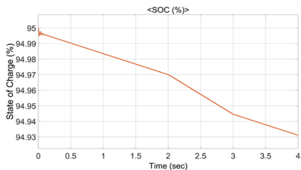
Fig. 8. Simulation analysis for the SOC (%).
