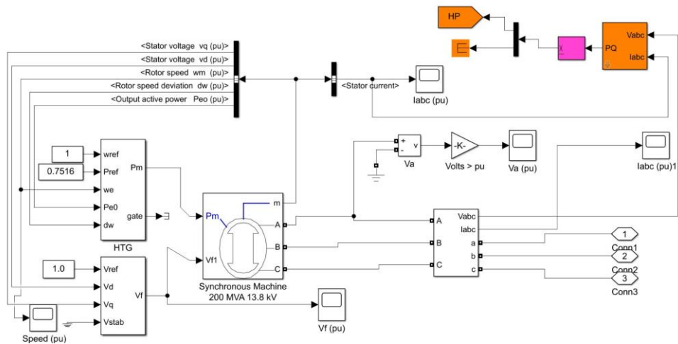
Fig. 2. Circuit modeling for pico hydro system.
