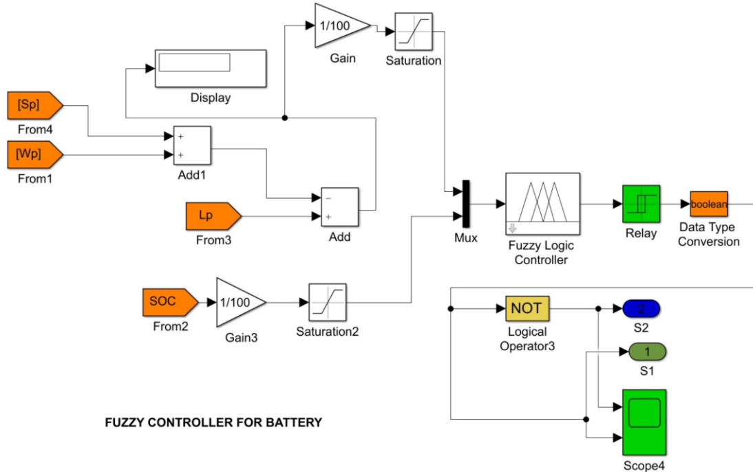
Fig. 5. BESS with fuzzy logic.
