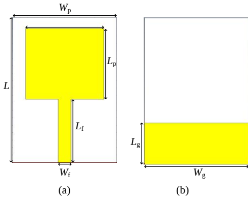
Fig. 1. Fundamental UWB antenna: (a) Top view and (b) Bottom view
